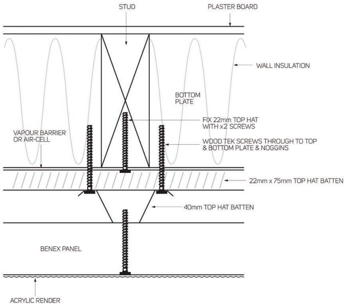
NOGGIN / BATTEN JUNCTION
